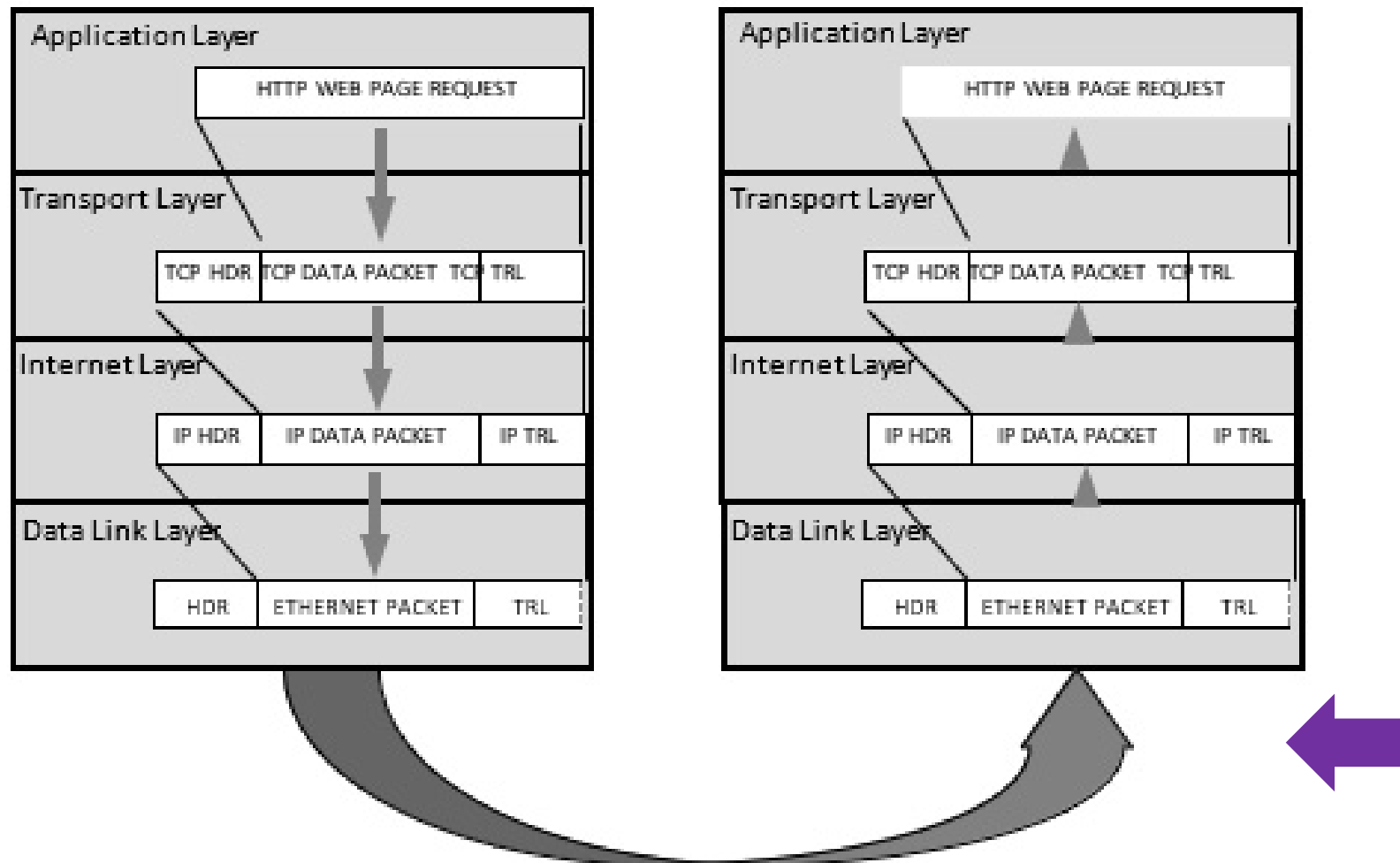
How TCP/IP Protocols Layer on Each Other
